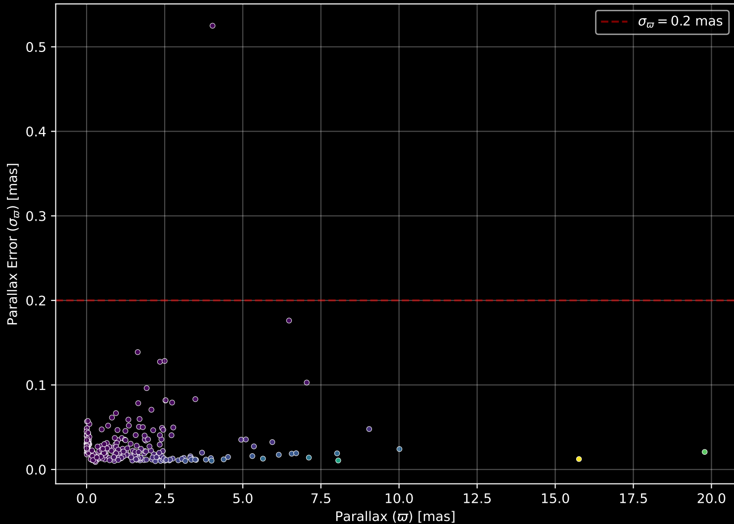
APOGEE DR17 Field: [LMC7] Parallax Quality (n= 288)
