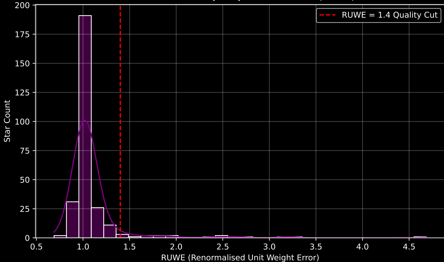
GAPOGEE DR17 Field [LMC7] RUWE Distribution (n= 278)
