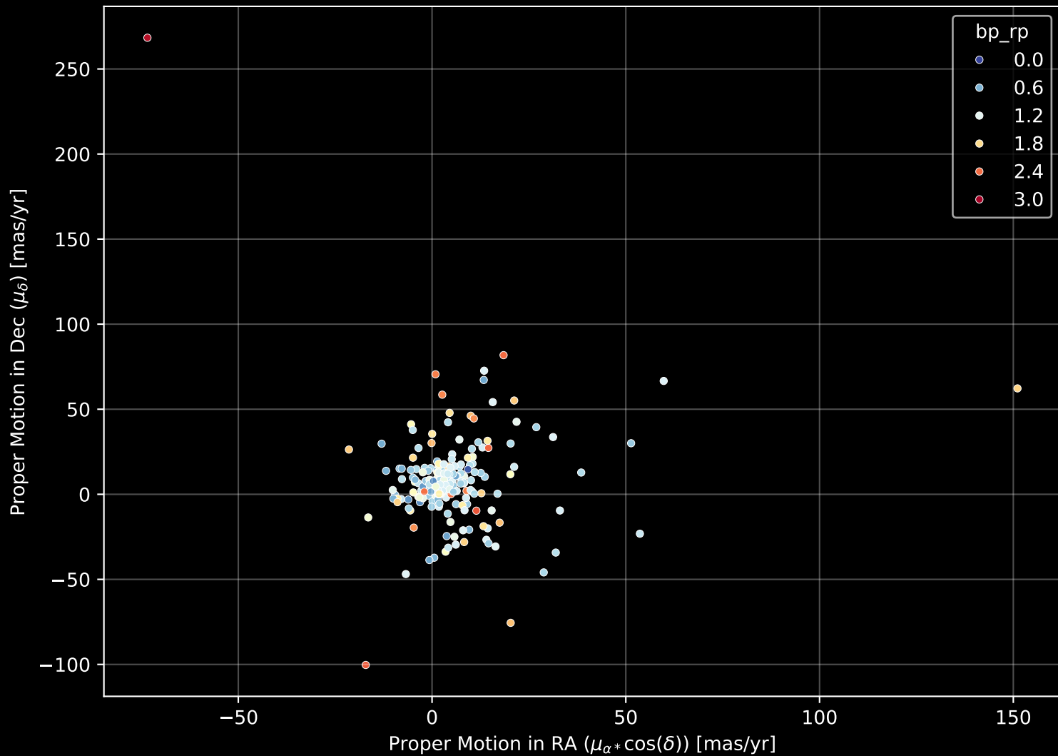
APOGEE DR17 Field: [LMC7] Proper Motion Diagram (n= 288)
