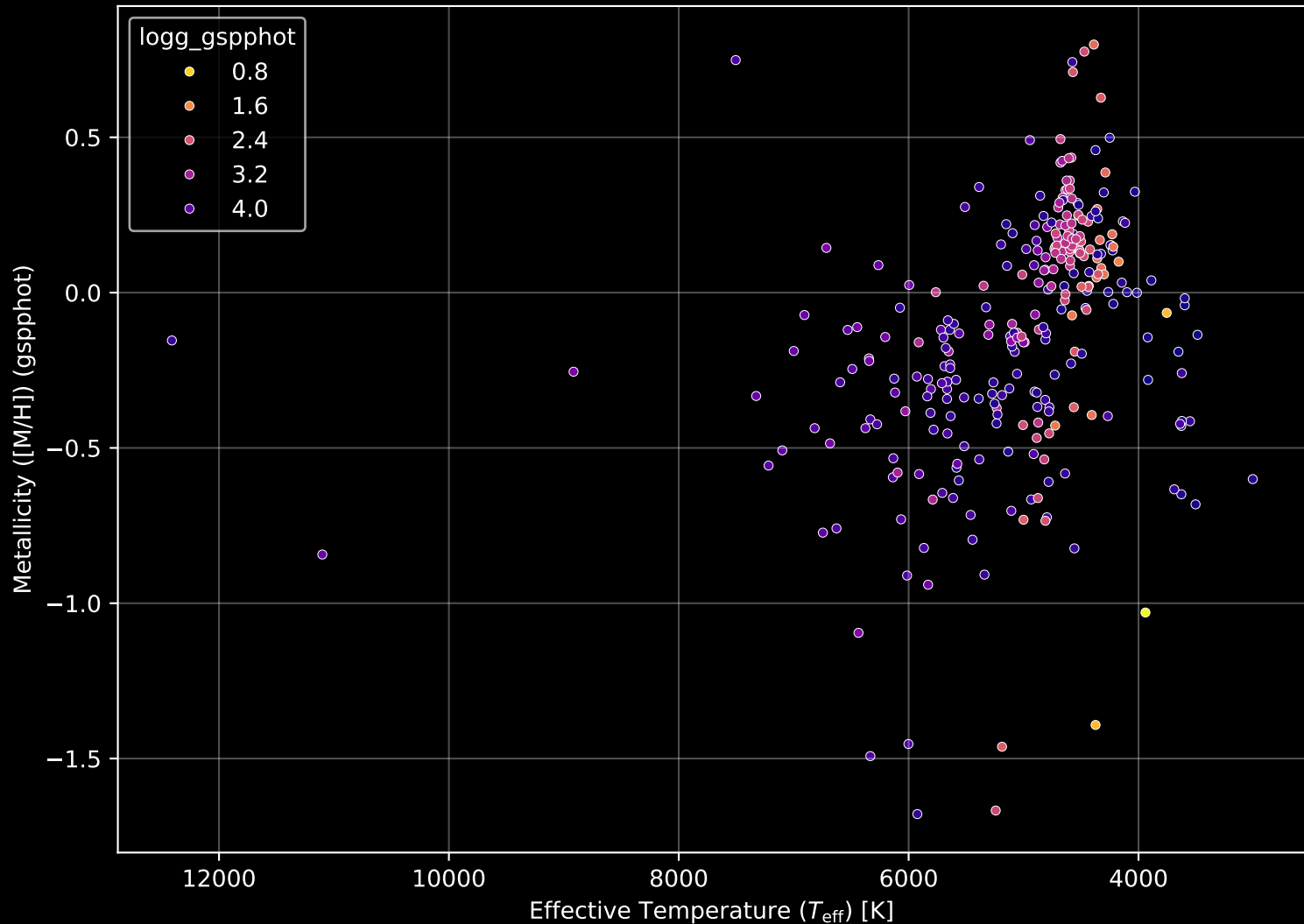
APOGEE DR17 Field: [LMC7] Stellar Population Parameters (n= 288)
