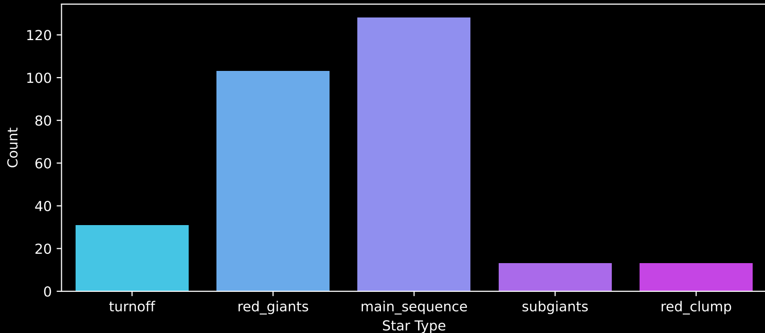
APOGEE DR17 Field: [LMC7] Count plot of Star Type
